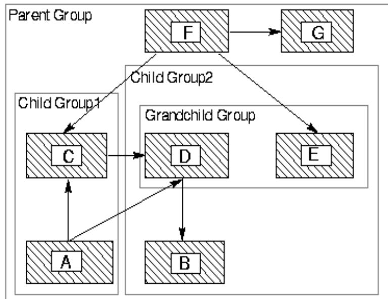
Figure 9: Groups visualized as nested regions
